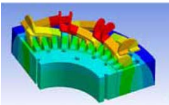
Steady-state temperature of a generator, eddy current, core and resistive losses from Maxwell imported into ANSYS Mechanical
