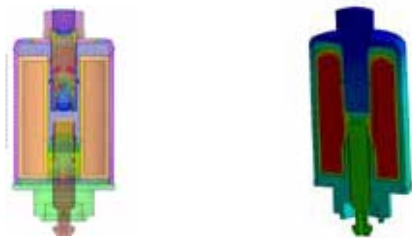
Solenoid actuator, magnetic flux results calculated in Maxwell (left) and steady-state temperature results (right) solved with ANSYS Mechanical
