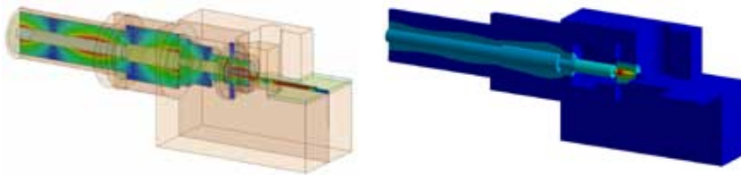
High-power connector, electric field results calculated in HFSS (left) and steady-state temperature results (right) solved with ANSYS Mechanical
